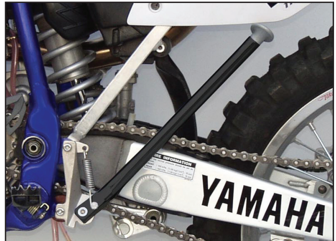
5201-PK Kickstand Installed
