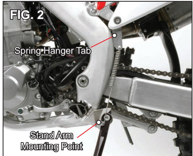
Kickstand Installed
